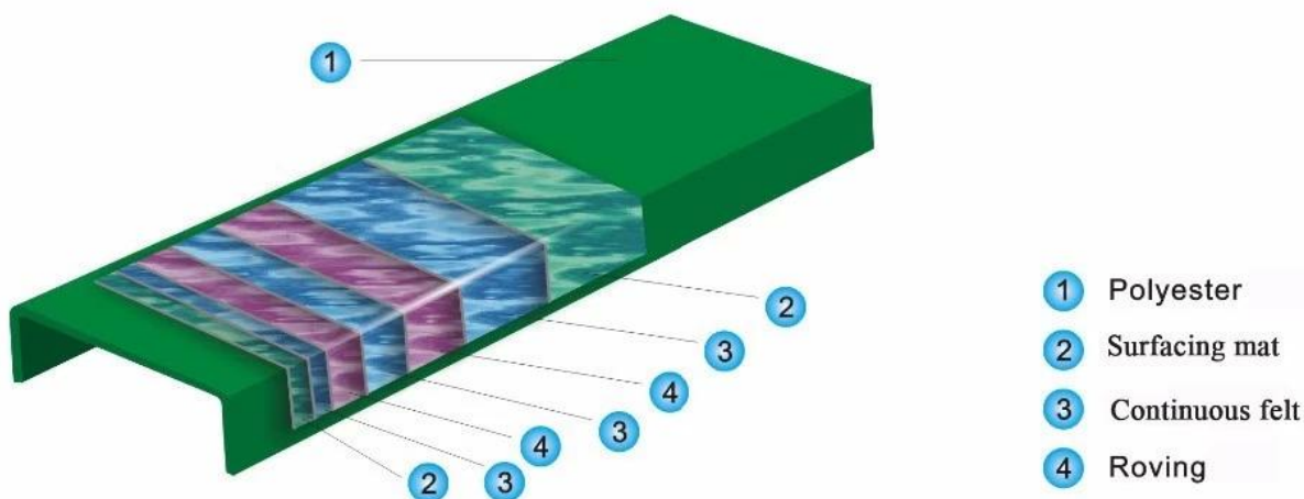
Structure chart
